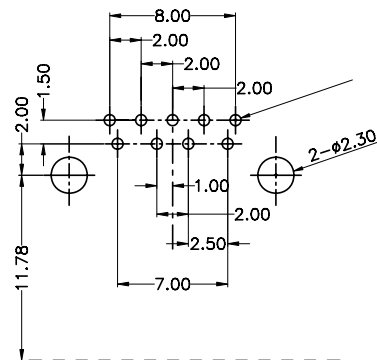
RECOMMENDED PCB LAYOUT(TOP VIEW) GENERAL TOLERANCES:±0.05
