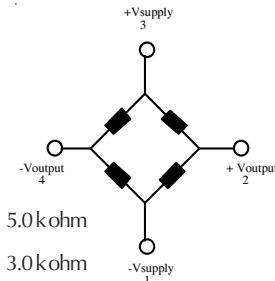
Equivalent Circuit
