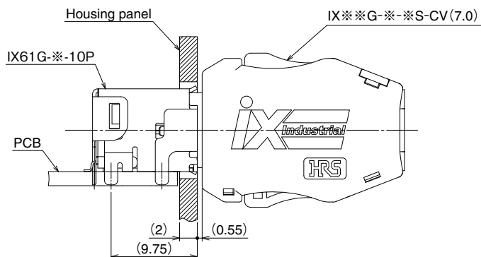
Mated Condition Diagram
