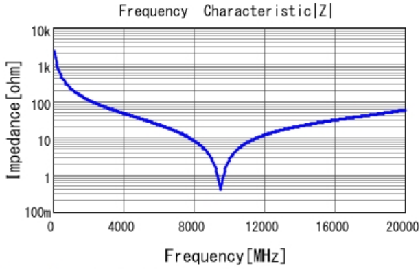
GJM1555C1HR70WB01 |Z| DCOV, 25degC
