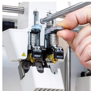
Print cores AA, BB, CC, and DD Quick-swap nozzles for support materials, abrasive materials, and metal printing
