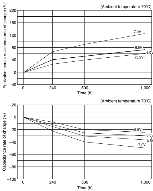
Fig. 43 FS0H473ZF Overvoltage Life Test
