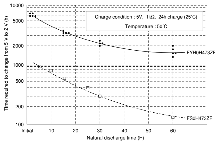
Fig. 16 Change of Self-Discharge Characteristic by Natural Discharge
