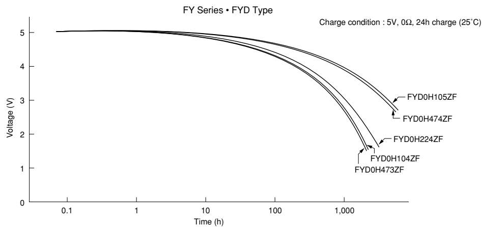
Fig. 15 Self-Discharge Characteristic
