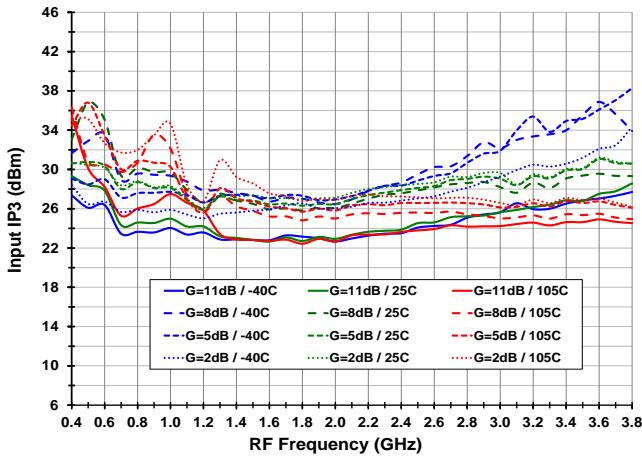
Figure 4. OIP3 vs. Temperature and Gain Setting
