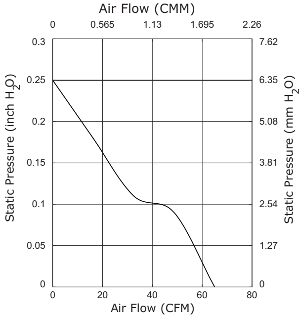
CFM-9225V-139-416
