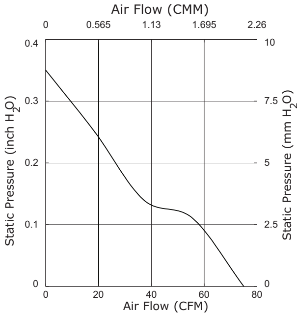
CFM-9225V-145-455
