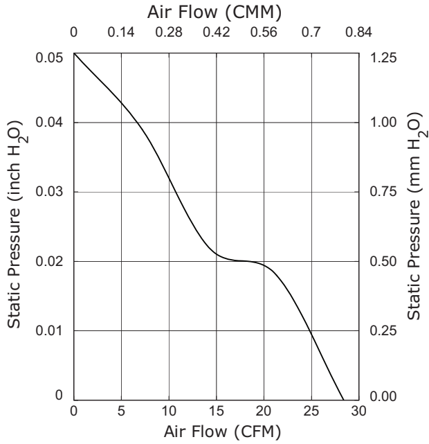
CFM-9225V-127-320
