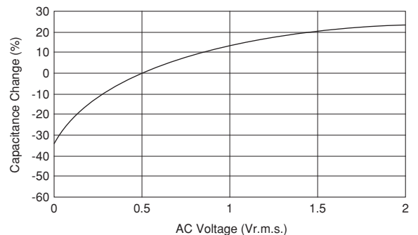
[AC Voltage Characteristics] Sample: X7R(R7) Characteristics 10μF, Rated Voltage 6.3VDC
