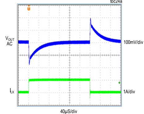
MAX17503S, 5V OUTPUT, PWM MODE, FIGURE 4c CIRCUIT (LOAD CURRENT STEPPED FROM NO LOAD TO 1A)
