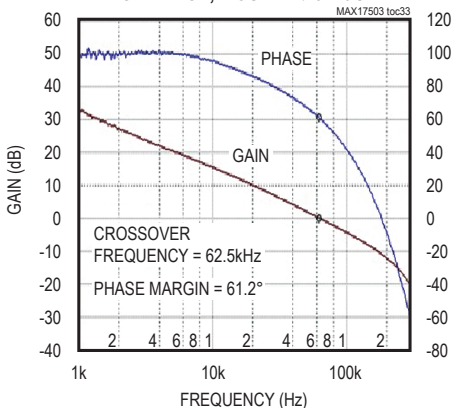
MAX17503 5V OUTPUT, 2.5A LOAD CURRENT BODE PLOT, FIGURE 4b CIRCUIT
