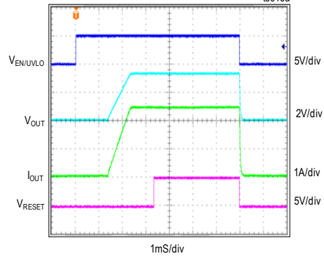
MAX17503S, SOFT-START/ SHUTDOWN FROM EN/UVLO, 3.3V OUTPUT, 2.5A LOAD CURRENT, FIGURE 4d CIRCUIT)
