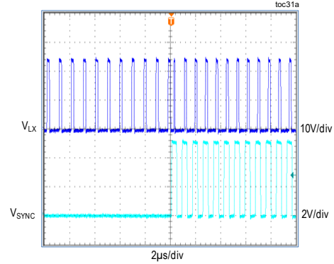
MAX17503S, APPLICATION OF EXTERNAL CLOCK AT 1.2MHz, 5V OUTPUT, FIGURE 4c CIRCUIT
