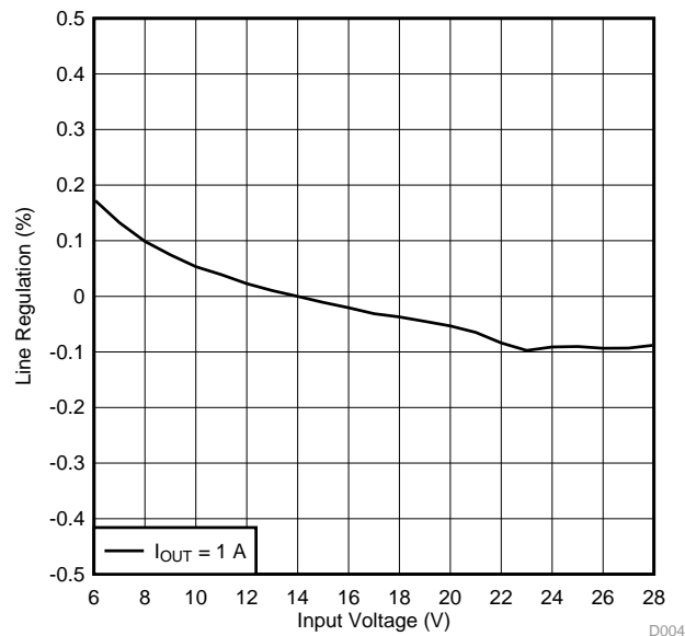
Figure 4. TPS54202EVM-716 Line Regulation
