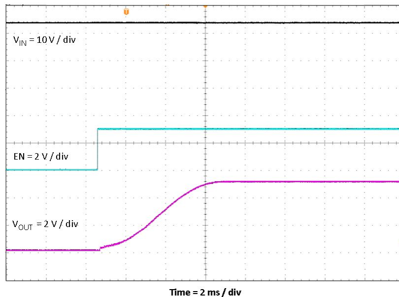
Figure 12. TPS54202EVM-716 Startup Relative to Enable
