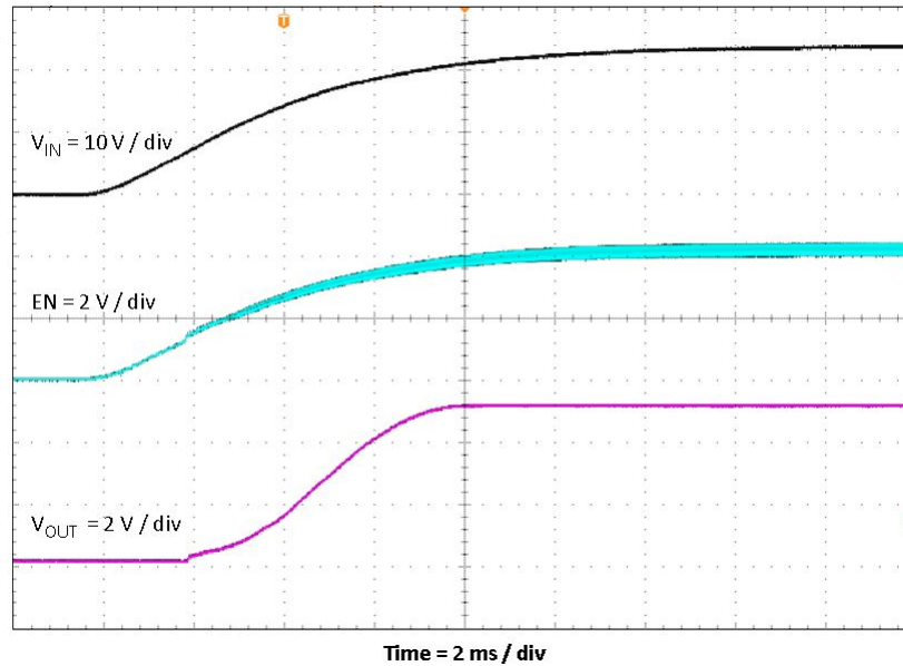
Figure 11. TPS54202EVM-716 Startup Relative to V_{IN}
