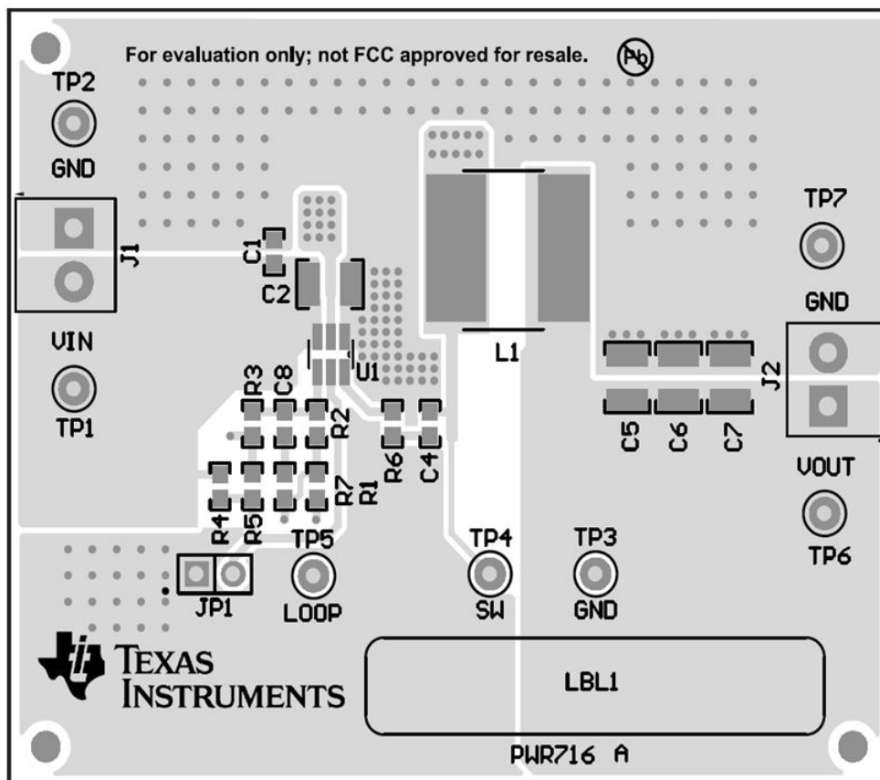
Figure 15. TPS54202EVM-716 Top-Side Assembly
