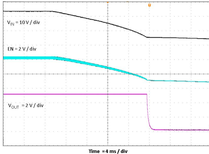
Figure 13. TPS54202EVM-716 Shutdown Relative to V_{IN}
