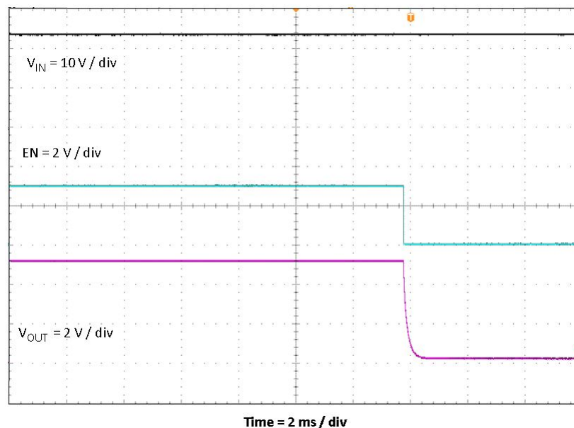
Figure 14. TPS54202EVM-716 Shutdown Relative to EN
