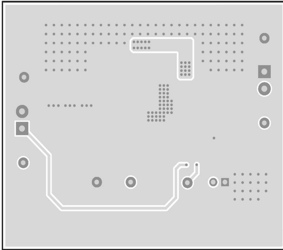
Figure 16. TPS54202EVM-716 Bottom-Side Layout
