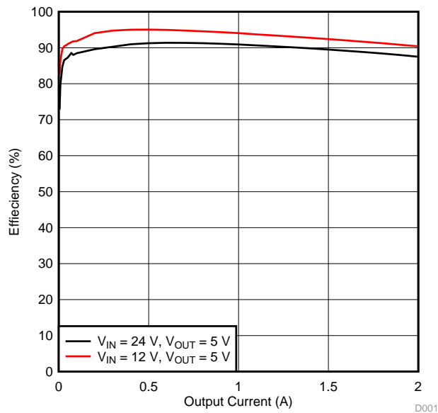
Figure 1. TPS54202EVM-716 Efficiency
