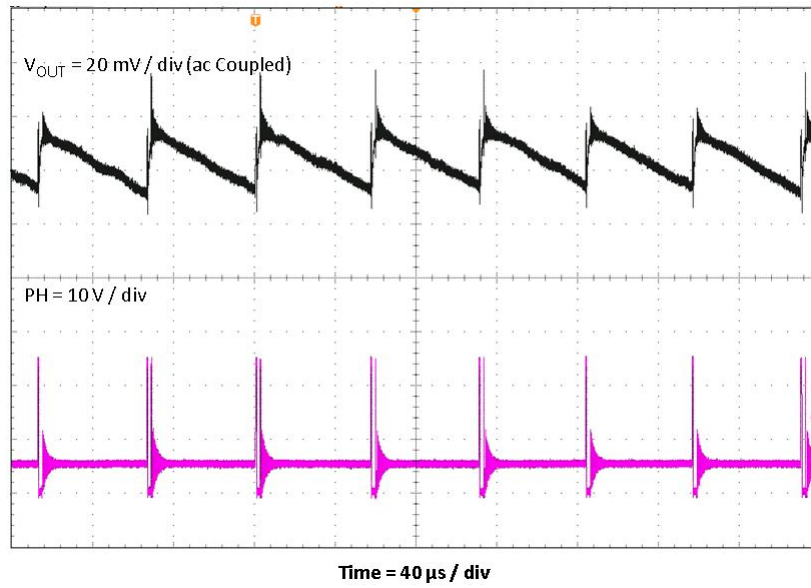
Figure 8. TPS54202EVM-716 Output Ripple, I_{OUT} = 10 \text{ mA}
