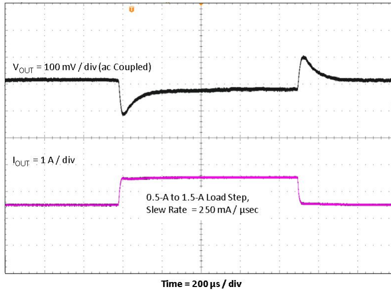
Figure 5. TPS54202EVM-716 Transient Response
