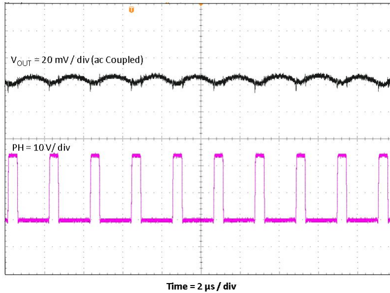
Figure 6. TPS54202EVM-716 Output Ripple, I_{OUT} = 2\text{ A}
