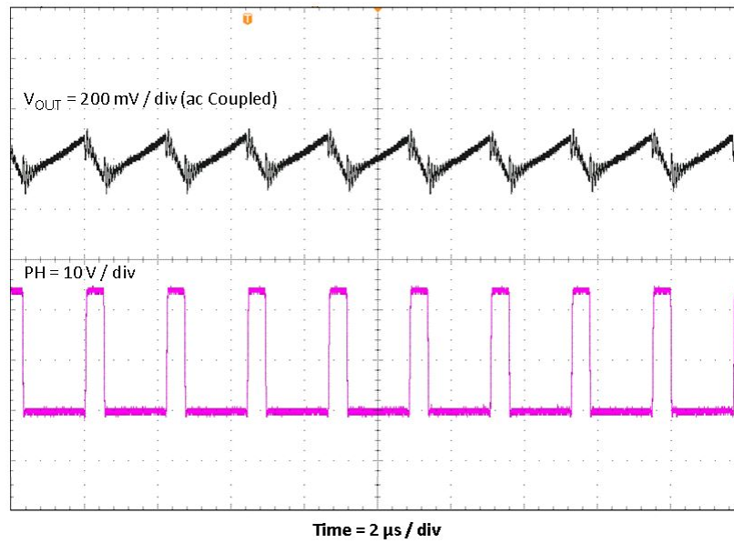
Figure 10. TPS54202EVM-716 Input Ripple
