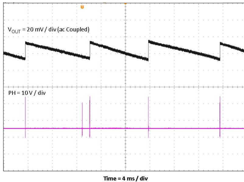
Figure 9. TPS54202EVM-716 Output Ripple, I_{OUT} = 0 \text{ A}
