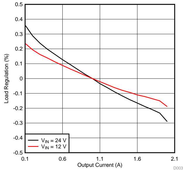
Figure 3. TPS54202EVM-716 Load Regulation
