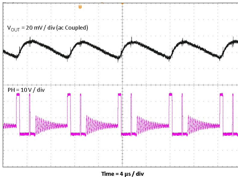
Figure 7. TPS54202EVM-716 Output Ripple, I_{OUT} = 100\text{ mA}
