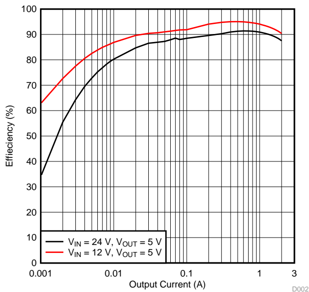
Figure 2. TPS54202EVM-716 Low Current Efficiency
