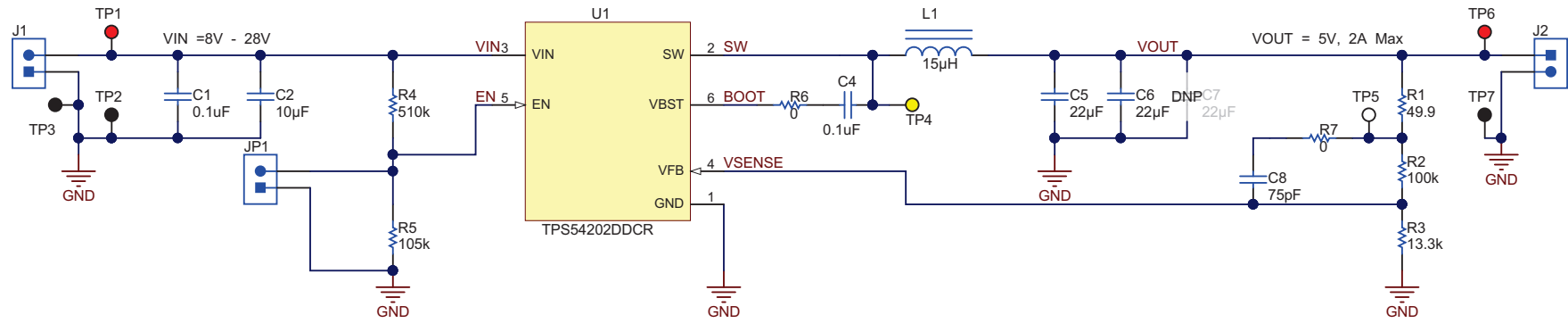
Figure 17. TPS54202EVM-716 Schematic
