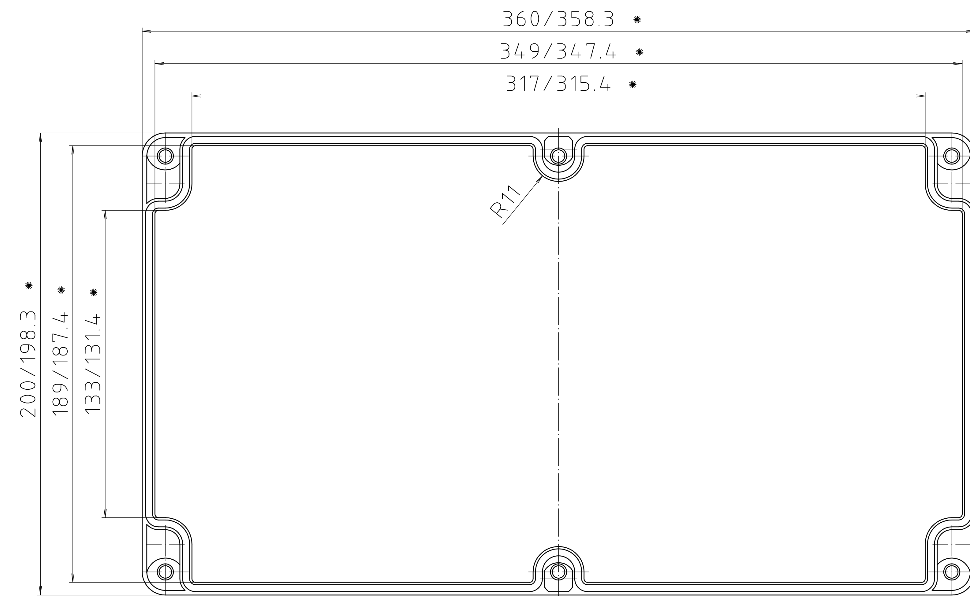
Deckel/lid
