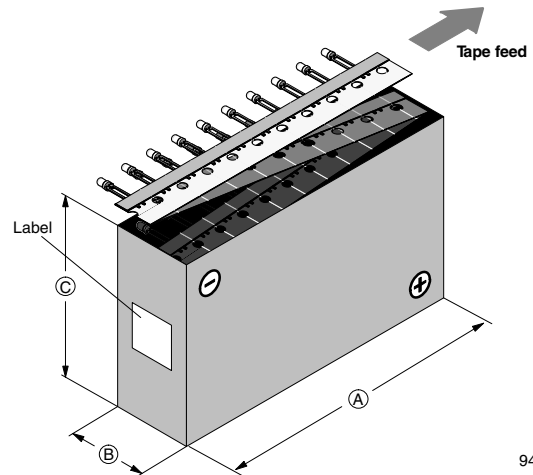
Fig. 20 - Tape Direction
