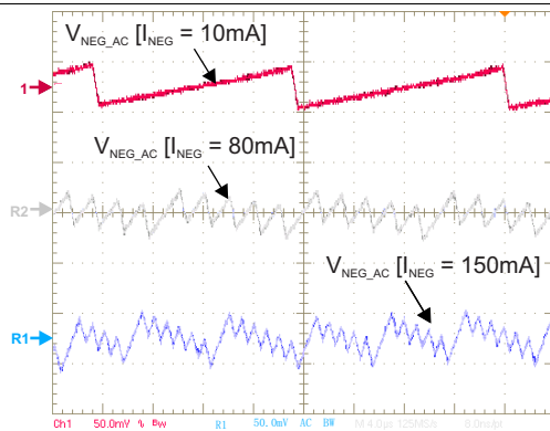
Figure 86. V_{\text{NEG}} Output Voltage Ripple — SYNC = HIGH — L = 2.2 \mu\text{H} — C_{\text{OUT}} = 10\text{ }\mu\text{F}
