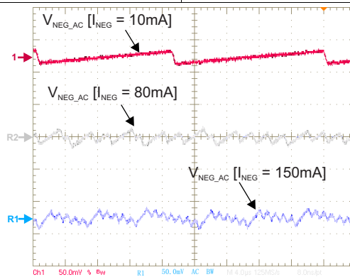
Figure 87. V_{\text{NEG}} Output Voltage Ripple — SYNC = HIGH — L = 2.2 \mu\text{H} — C_{\text{OUT}} = 2 \times 10\text{ }\mu\text{F}
