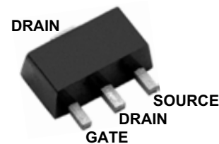
TO-243AA (SOT-89)
