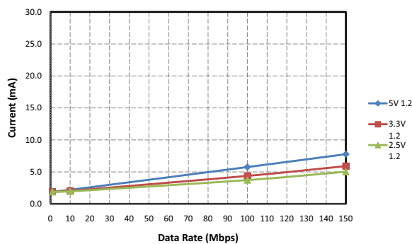
Figure 11. Si8621 Typical V_{DD1} or V_{DD2} Supply Current vs. Data Rate 5, 3.3, and 2.70 V Operation (15 pF Load)
