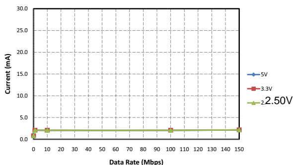
Figure 10. Si8620 Typical V_{DD1} Supply Current vs. Data Rate 5, 3.3, and 2.70 V Operation
