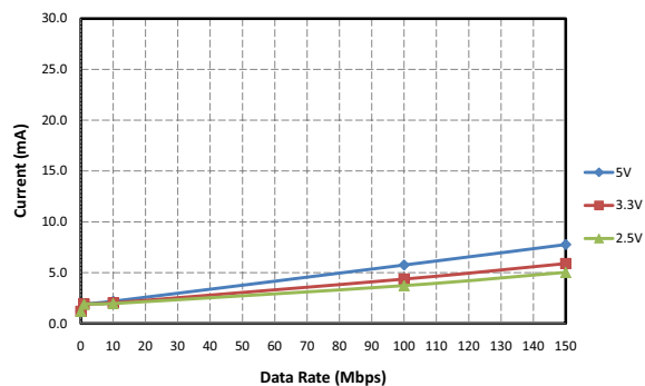
Figure 14. Si8622 Typical V_{DD1} or V_{DD2} Supply Current vs. Data Rate 5, 3.3, and 2.70 V Operation (15 pF Load)
