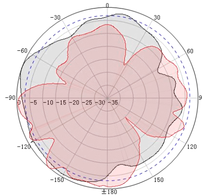
Figure 3 - E-Plane @ 1800MHz
