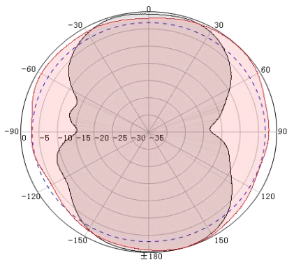
Figure 2 - E-Plane @ 2100MHz
