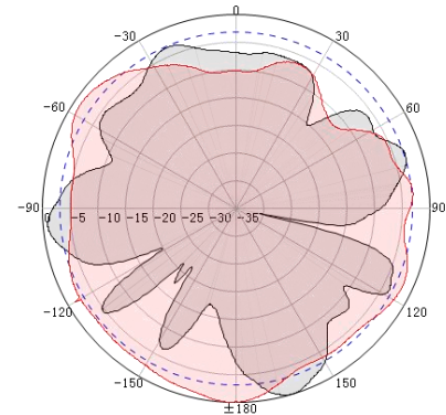
Figure 4 - E-Plane @ 920MHz
