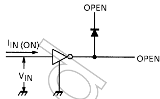
3. I_{IN(ON)}
