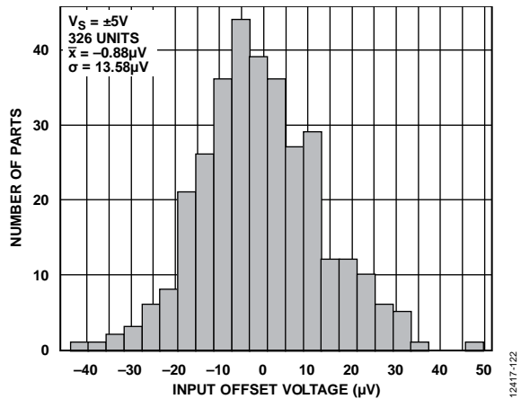
Figure 24. Input Offset Voltage
