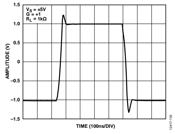
Figure 35. Large Signal Step Response (Differential Output), V_S = \pm 5\text{ V}
