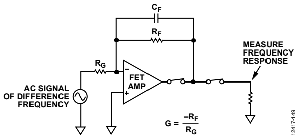
Figure 52. Frequency Response for FET Input Amplifier, Inverting Gain Configuration
