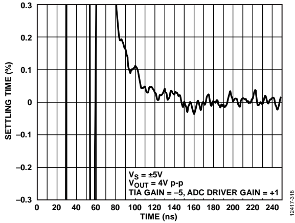
Figure 14. 0.1% Settling Time, See Test Circuit in Figure 50
