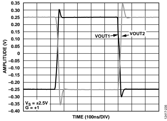
Figure 36. Large Signal Step Response (Single-Ended Output), V_S = \pm 2.5 V
