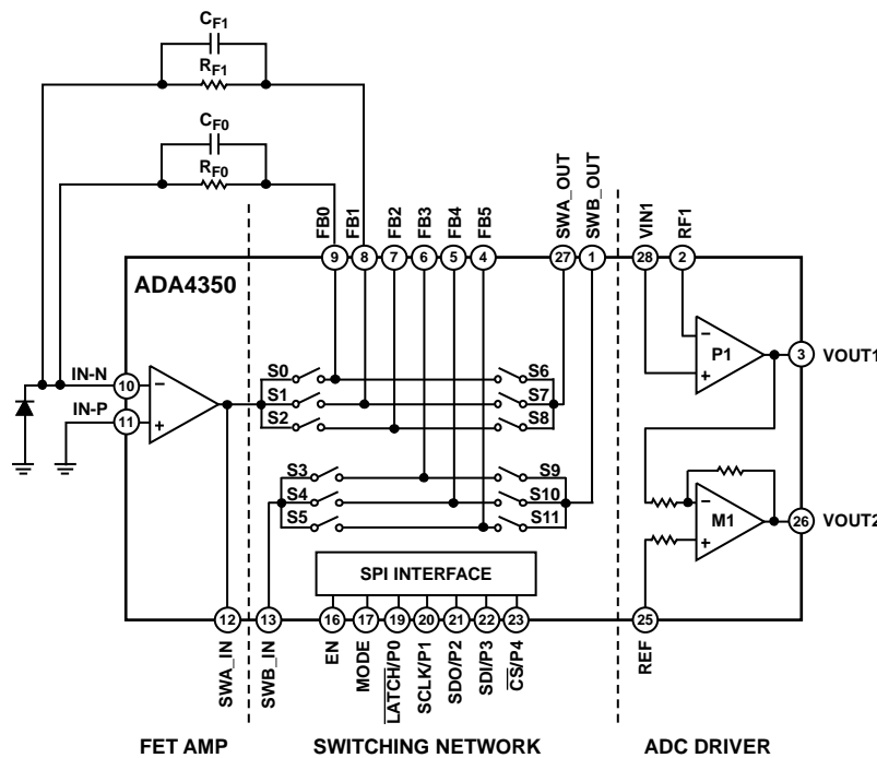
Figure 56. Simplified Schematic
