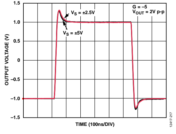
Figure 20. Large Signal Step Response for Various Supplies, G = -5
