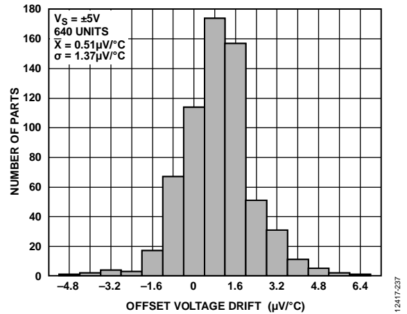
Figure 40. Differential Output Offset Voltage Drift
