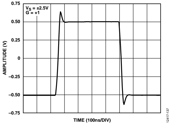
Figure 37. Large Signal Step Response (Differential Output), V_S = \pm 2.5 V
