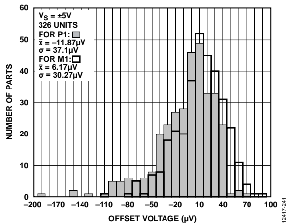
Figure 41. Single-Ended Output Offset Voltage
