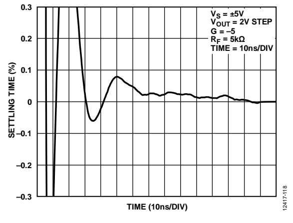
Figure 21. 0.1% Settling Time
