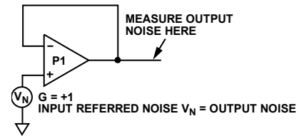
Figure 53. Input Referred Voltage Noise for P1
