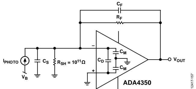
Figure 59. Transimpedance Amplifier Model of the ADA4350
