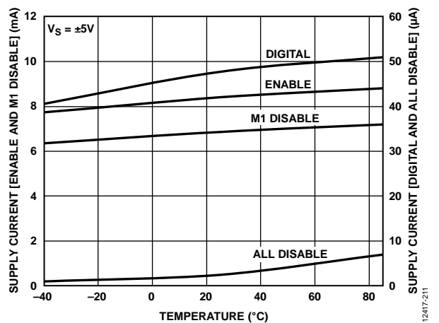
Figure 12. Supply Current vs. Temperature at Different Modes
