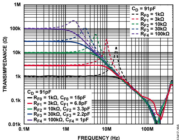
Figure 63. Transimpedance vs. Frequency, C_D = 91 pF
