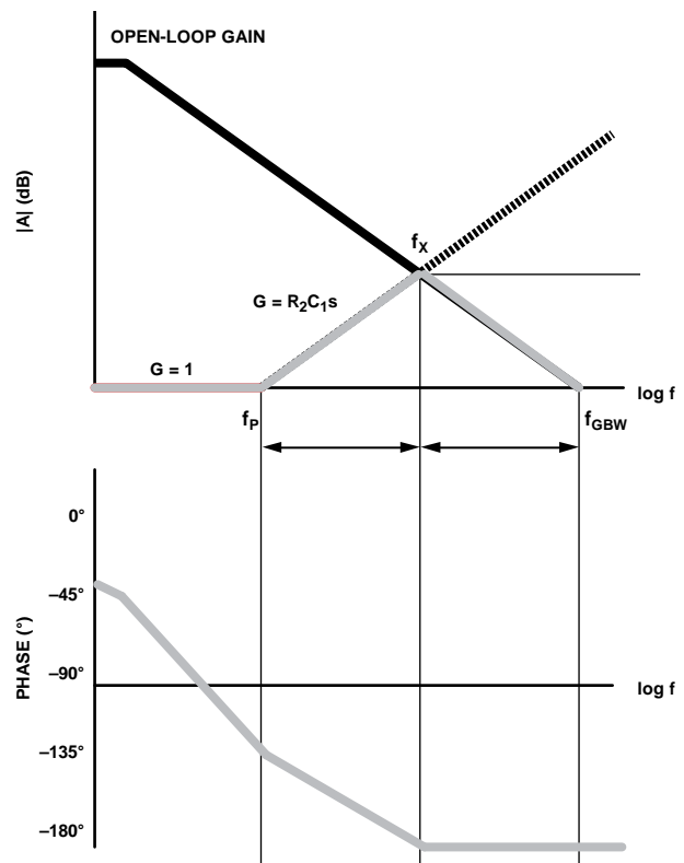
Figure 60. Noise Gain and Phase Bode Plot of the Transimpedance Amplifier Design Without Compensation
