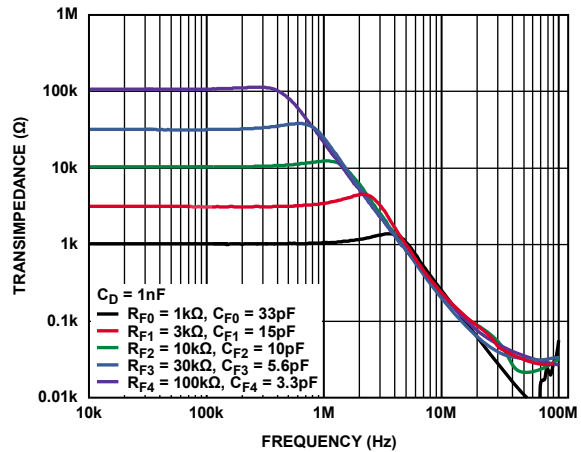
Figure 64. Transimpedance vs. Frequency, C_D = 1 nF
