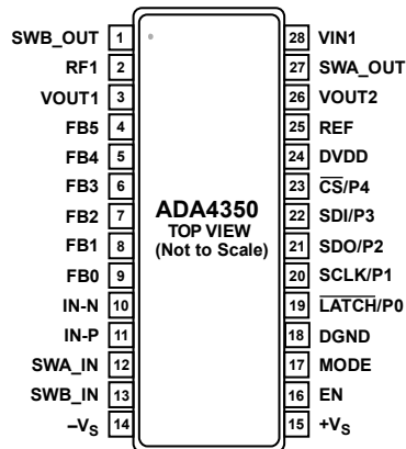
Figure 6. Pin Configuration
