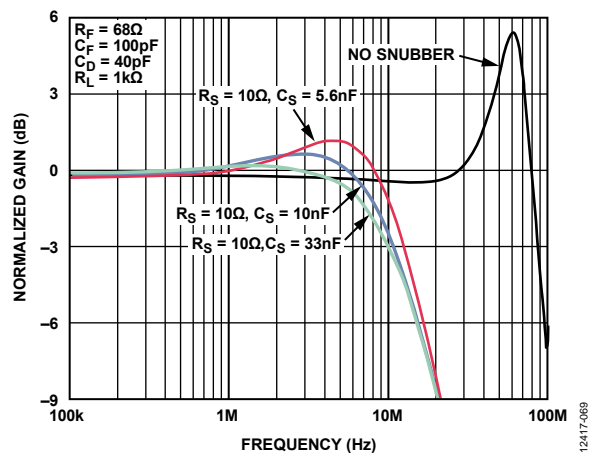
Figure 70. Effect of Snubber Circuits on the Transimpedance Frequency Response (See Figure 69)
