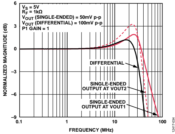
Figure 30. Small Signal Frequency Response, V_S = 5\text{ V}
