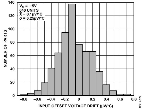
Figure 25. Input Offset Voltage Drift
