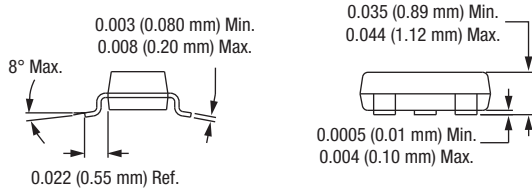
Figure 7. SOT-23 Package Dimensions
