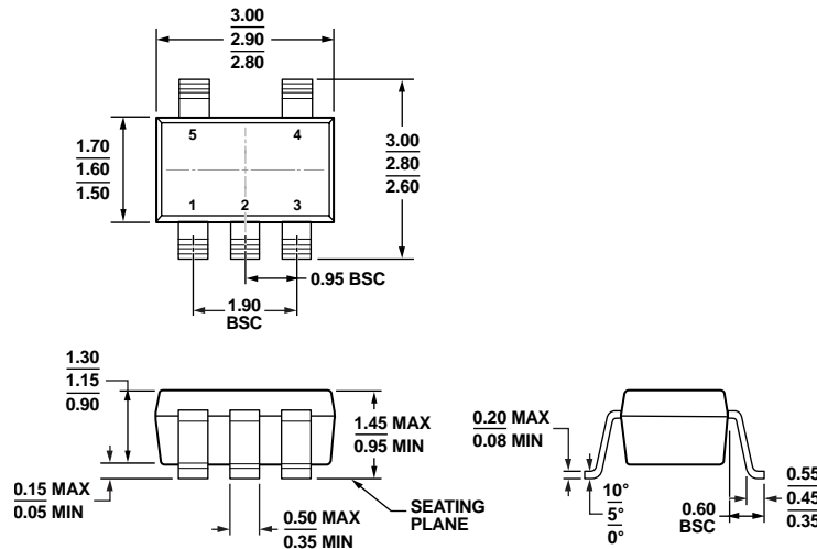
COMPLIANT TO JEDEC STANDARDS MO-178-AA Figure 26. 5-Lead Small Outline Transistor Package [SOT-23] (RJ-5)
