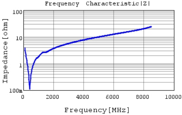
GRM1555C1E391JA01 |Z| DCOV, 25degC
