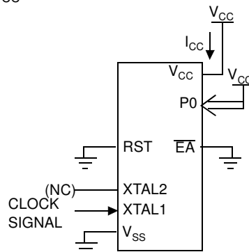
Figure 25-2. I_{CC} Test Condition, Idle Mode
