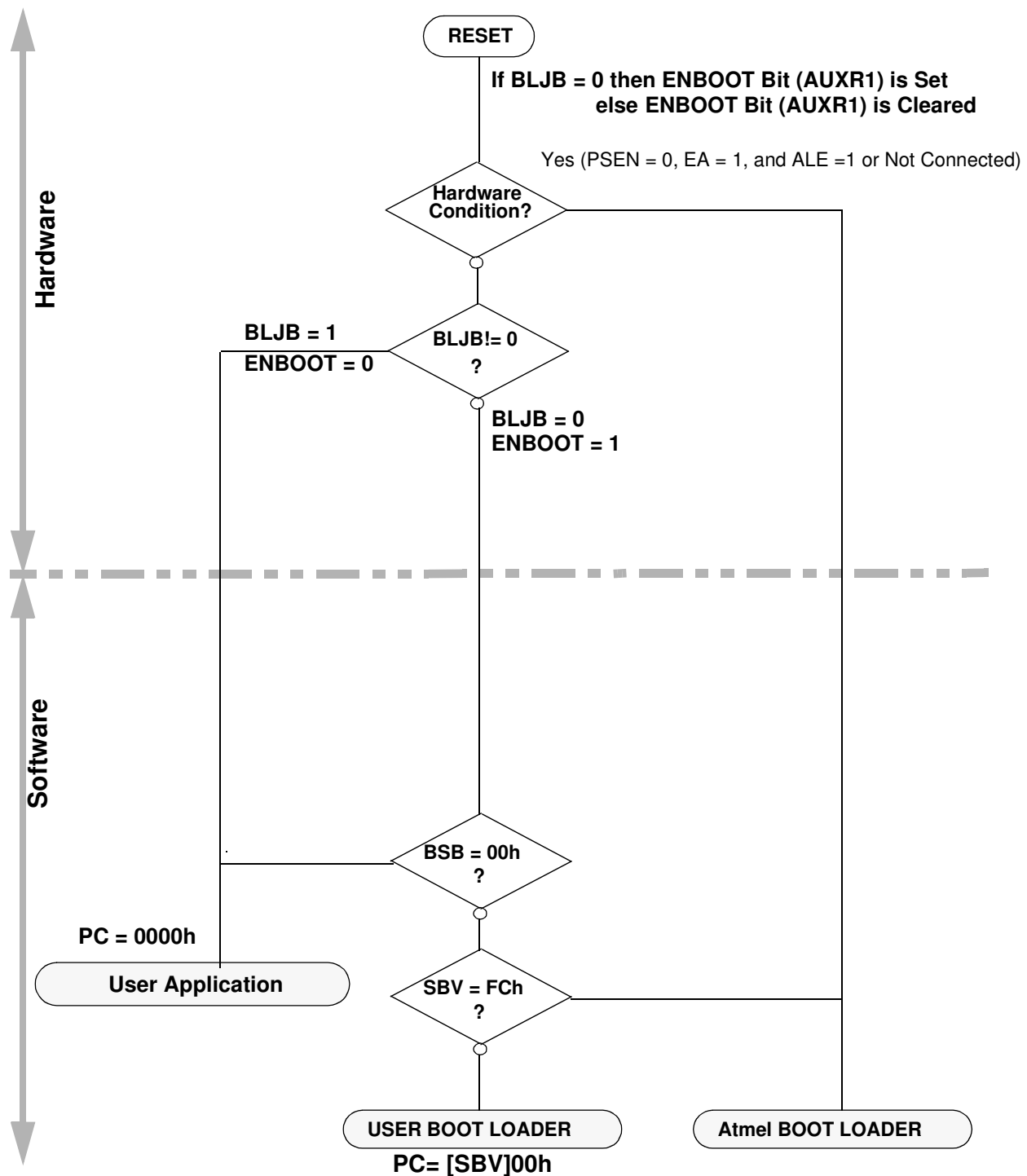
Figure 24-5. Bootloader Process
