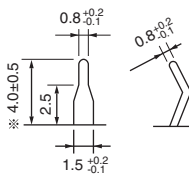
(Terminal dimensions)
