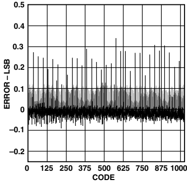
Figure 34. Typical DNL
