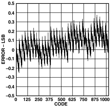
Figure 33. Typical INL
