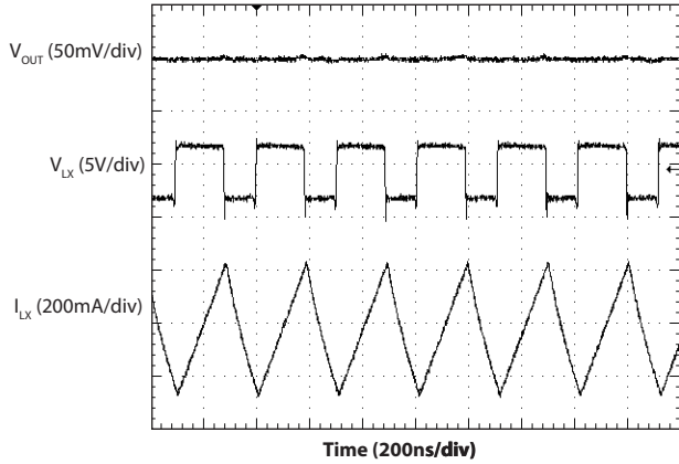
Heavy Load Switching — V_{OUT} = 2.8V
