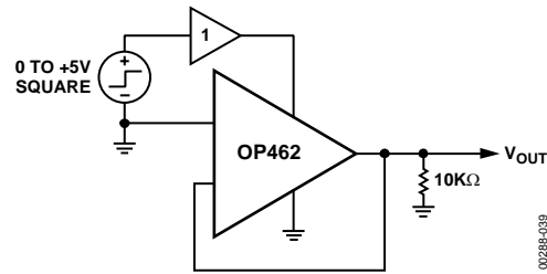
Figure 36. Test Circuit for Power-On Settling Time
