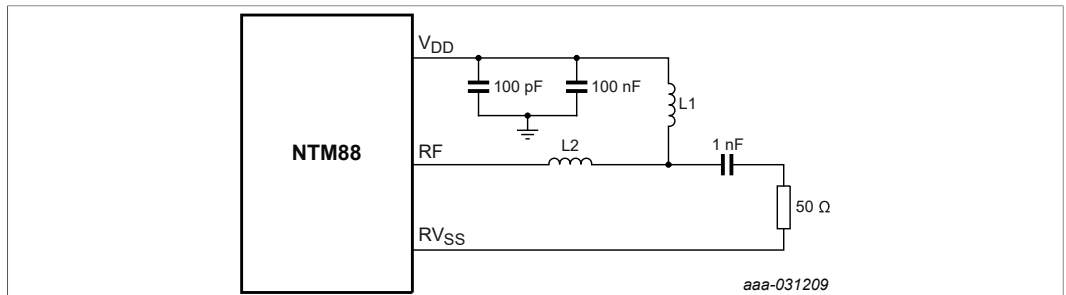
Figure 6. RF output power measurement configuration
