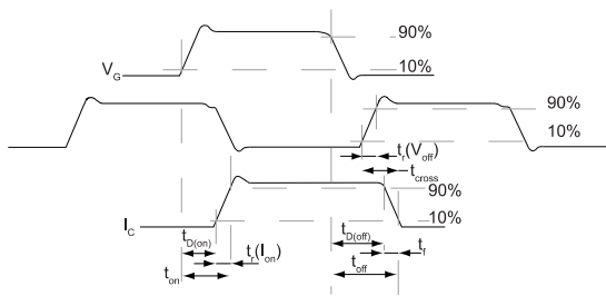
Figure 31: Switching waveform
