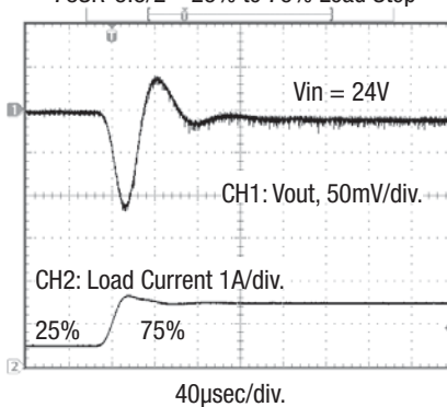
78SR-5/2 25% to 75% Load Step
