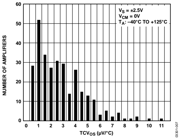
Figure 7. TCVos Distribution
