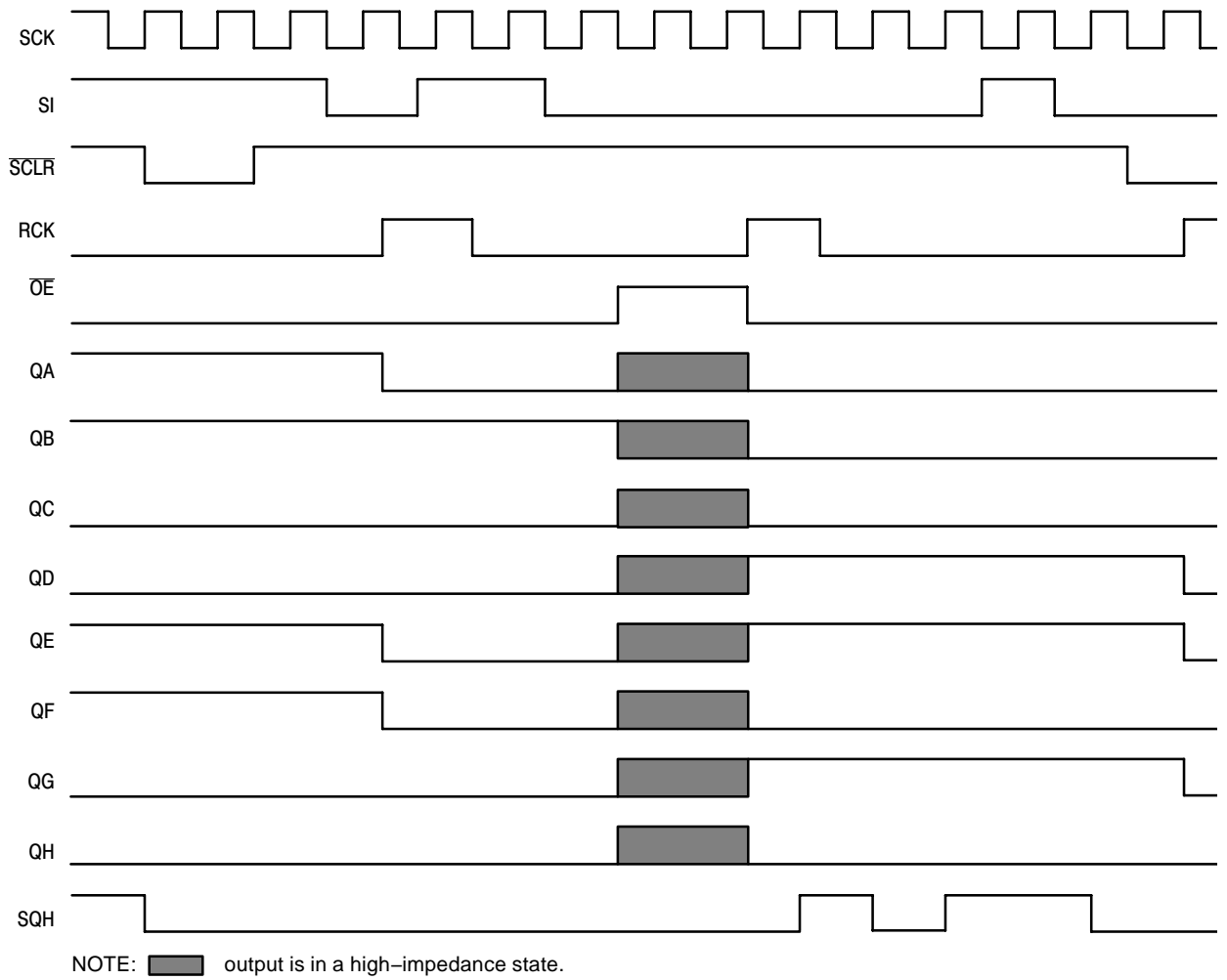
Figure 14. Timing Diagram
