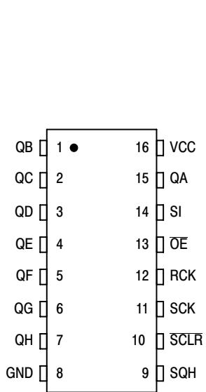
Figure 1. Pin Assignment (TSSOP-16)
