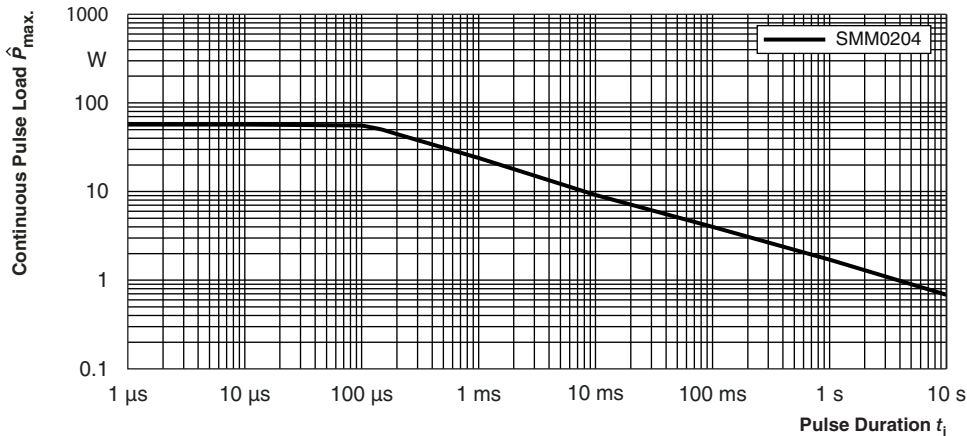
Maximum pulse load, continuous pulse; applicable if \hat{P} \leq P(\vartheta_{amb}) and \hat{U} \leq \hat{U}_{max,i} ; for permissible resistance change \pm (0.5\% R + 0.01 \Omega)
