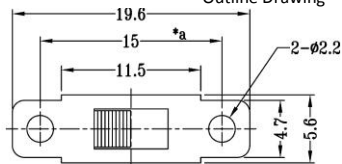
Outline Drawing
