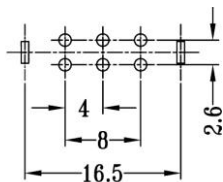
Mounting
