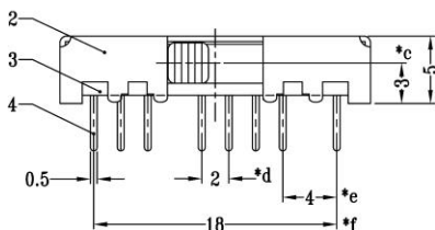
Mounting
