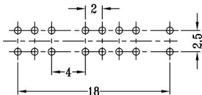
Mounting
