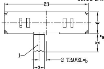
Outline Drawing
