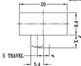
Outline Drawing
