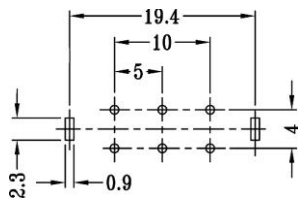
Mounting
