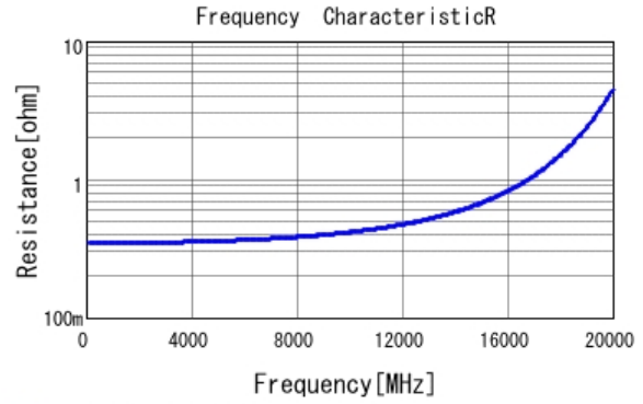
■ GJM1555C1HR40WB01 R DCOV, 25degC
