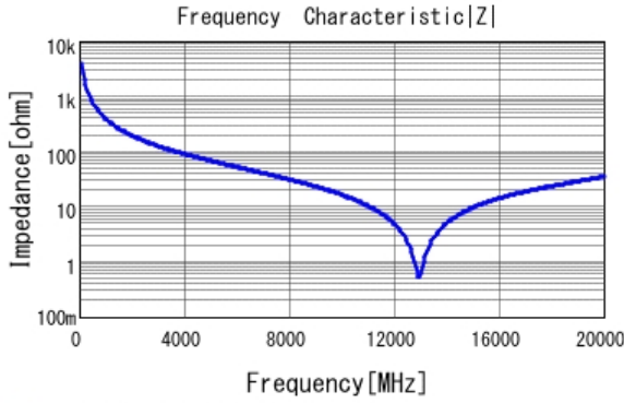
■ GJM1555C1HR40WB01 |Z| DCOV, 25degC
