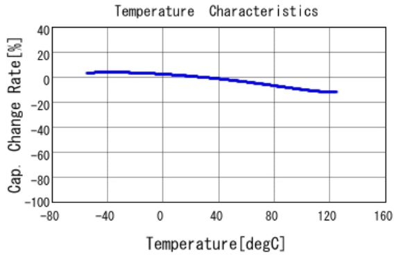
■ GRM033R70J472KA01 C-Temp. capchange, DC0.0V, AC1.0Vrm
