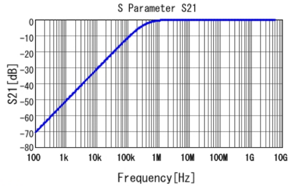
■ GRM033R70J472KA01 S21 DC0V, 25degC
