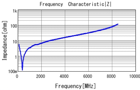
■ GRM1885C2A271JA01 |Z| DCOV, 25degC
