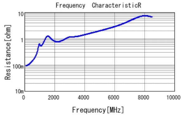
■ GRM1885C2A271JA01 R DCOV, 25degC
