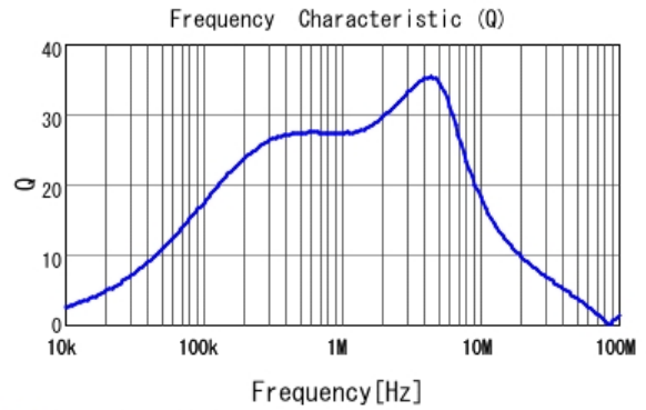
■ LQH44PN2R2MP0 Q
