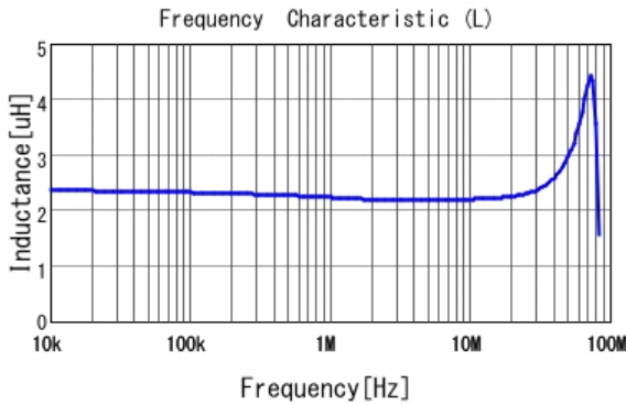
■ LQH44PN2R2MP0 L
