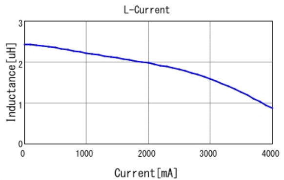
■ LQH44PN2R2MP0 L-Current 20degC
