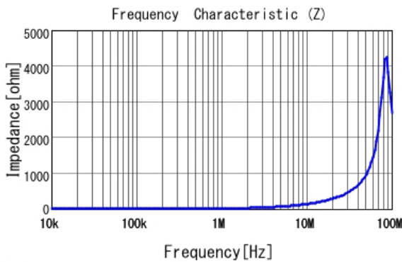
■ LQH44PN2R2MP0 |Z|
