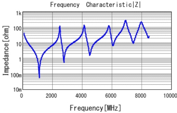
■ GQM22M5C2H390JB01 |Z| DC0V, 25degC
