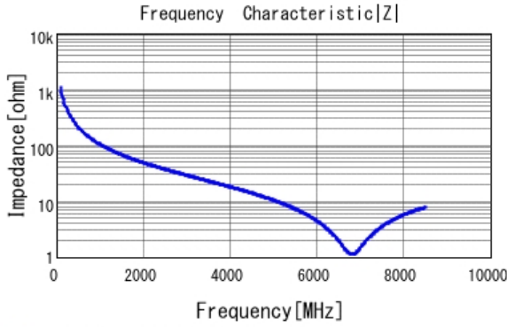
■ GRM1555C1H1R5WA01 |Z| DC0V, 25degC
