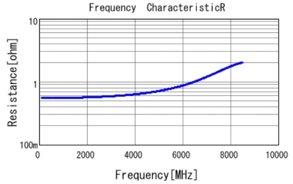
■ GRM1555C1H1R5WA01 R DC0V, 25degC
