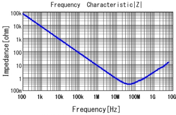
■ GCJ188R72A223KA01 |Z| DCOV, 25degC
