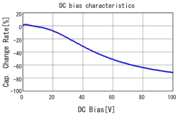
■ GCJ188R72A223KA01 C-DC bias capchange, 25.0degC, AC1.
