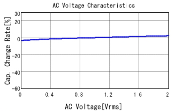
■ GCJ188R72A223KA01 C-AC Voltage capchange, DCOV, 25.0d
