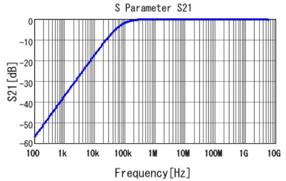
■ GCJ188R72A223KA01 S21 DC0V, 25degC
