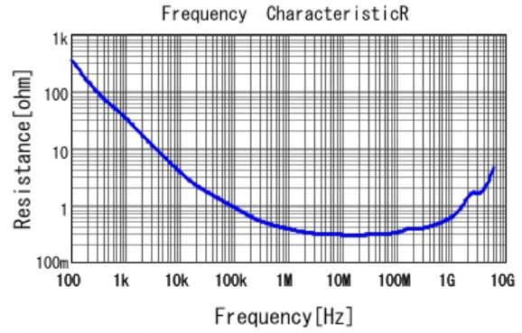
■ GCJ188R72A223KA01 R DCOV, 25degC
