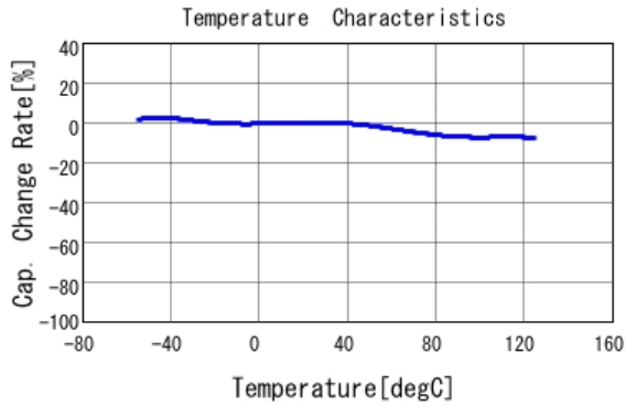
■ GCJ188R72A223KA01 C-Temp. capchange, DC0.0V, AC1.0V rm
