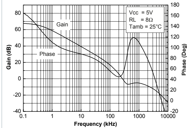
Figure 2. Open loop gain and phase vs. frequency
