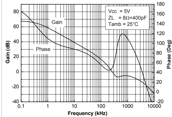
Figure 4. Open loop gain and phase vs. frequency V_{CC} = 5V
