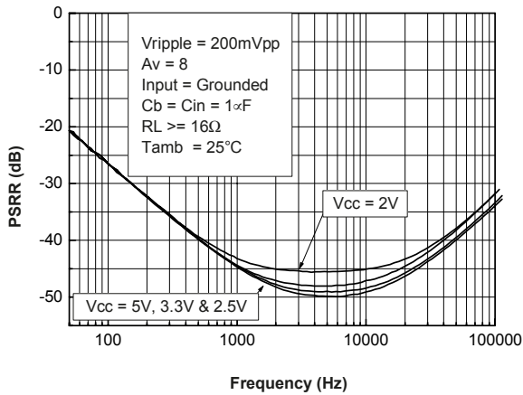
Figure 95. PSRR vs. bypass capacitor Cb = Cin = 1 μF
