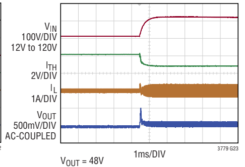
Line Transient Rising Edge
