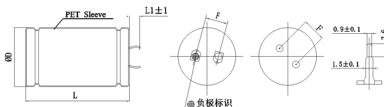
盖板型超级电容器示意图 Shape of snap-in and lead types supercapacitor:
