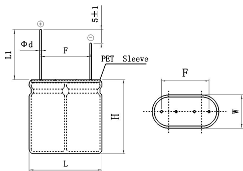
两端引出式示意图 Shape of wire lead supercapacitor:
