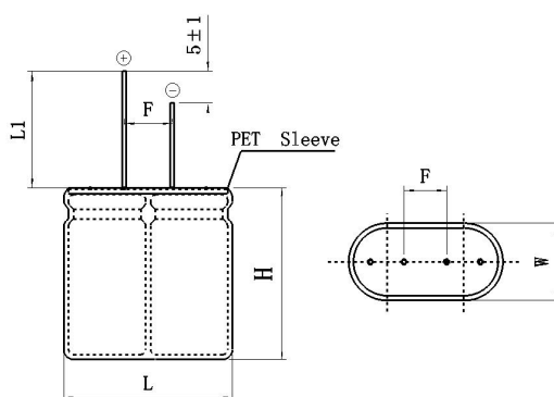
中间引出式示意图 Shape of snap in and lead types supercapacitor:
