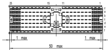
Board hole pattern (Component mounting side)
