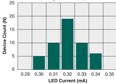
Typical I F for Switch Operation (N=50, I L =120mA, T A =25°C)
