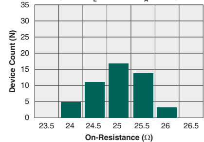
Typical On-Resistance Distribution (N=50, I L =120mA, T A =25°C)
