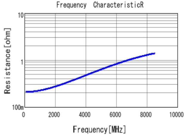
■ GRM0335C1H5R0BA01 R DCOV, 25degC
