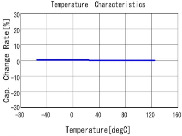
■ GRM0335C1H5R0BA01 C-Temp. capchange, DCOV, AC1Vrms
