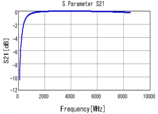
■ GRM0335C1H5R0BA01 S21 DCOV, 25degC
