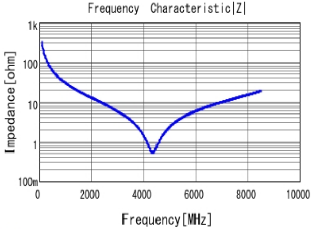
■ GRM0335C1H5R0BA01 |Z| DCOV, 25degC
